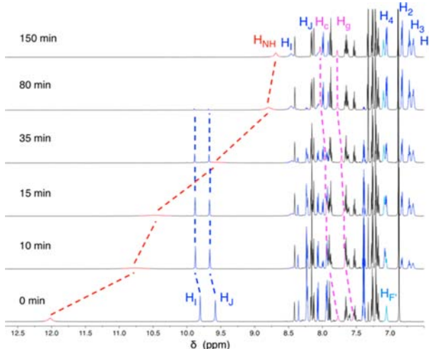
Figure 2. 1 H NMR spectra (300 MHz, CD 2 Cl 2 , 298 K) of a mixture of 1 , B , and 2 (1:1:0.5, [ B ] = 2 mM) after irradiation ( \lambda = 350\text{--}400 nm) for 0, 10, 15, 35, 80, and 150 min.
