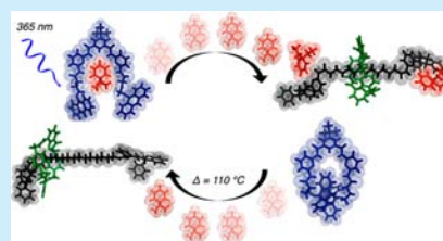
Scheme 1. Supramolecular System Where Photoregulated Binding of a Barbiturate Messenger Modulates the Amplitude of the Translational Motion of a Ring in an Interlocked Architecture
