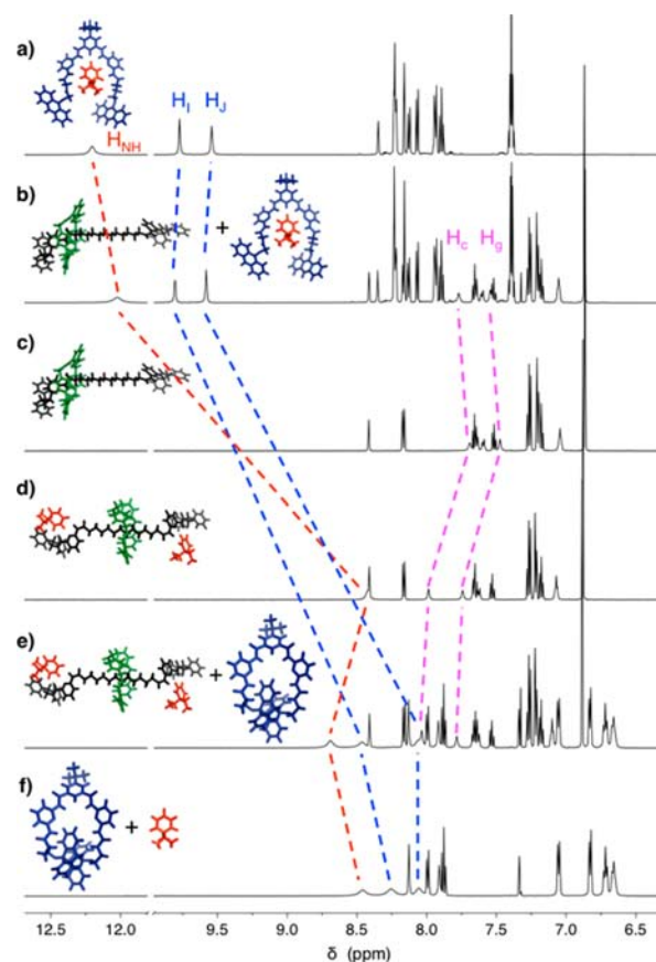
Figure 1. Partial 1 H NMR spectra (600 MHz, CD 2 Cl 2 , 298 K) of (a) a mixture of 1 and B (1:1, [ B ] = 2 mM); (b) a mixture of 1 , B and 2 (1:1:0.5, [ B ] = 2 mM); (c) 2 (1 mM), (d) complex 2B·2 (1:0.5, 2 mM); (e) mixture of 1 C , B , and 2 (1:1:0.5, 2 mM); (f) mixture of 1 C and B (1:1, [ B ] = 2 mM). Assigned resonances correspond to labeled protons in Scheme 1 (see the Supporting Information for full attribution). Space-filling structures generated by PM6 modeling.
