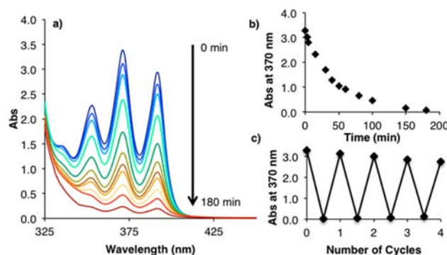
Figure 4. (a) Electronic absorption spectra (1 mm path length) of a mixture of 1 , B , and 2 (1:1:0.5, [\text{B}] = 2 \text{ mM} ) in \text{CH}_2\text{Cl}_2 . On irradiation ( \lambda = 350\text{--}400 \text{ nm} ), the disappearance of the anthracene moieties ( \text{Abs}_{370 \text{ nm}} , b) continued to 94% conversion. (c) Cycles of photoirradiation and thermal reversion, corresponding to shuttling of B between 1 and 2 .
