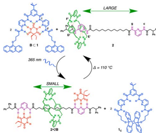
Scheme 1. Supramolecular System Where Photoregulated Binding of a Barbiturate Messenger Modulates the Amplitude of the Translational Motion of a Ring in an Interlocked Architecture
