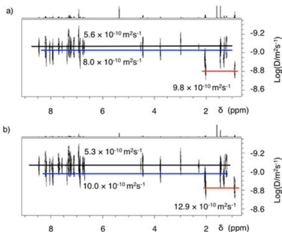
Figure 3. DOSY NMR spectra (600 MHz, \text{CD}_2\text{Cl}_2 , 298 K) of a mixture of 1 , B , and 2 (1:1:0.5, [\text{B}] = 2 \text{ mM} ): (a) before irradiation; (b) after irradiation ( \lambda = 350\text{--}400 \text{ nm} ) for 150 min.
